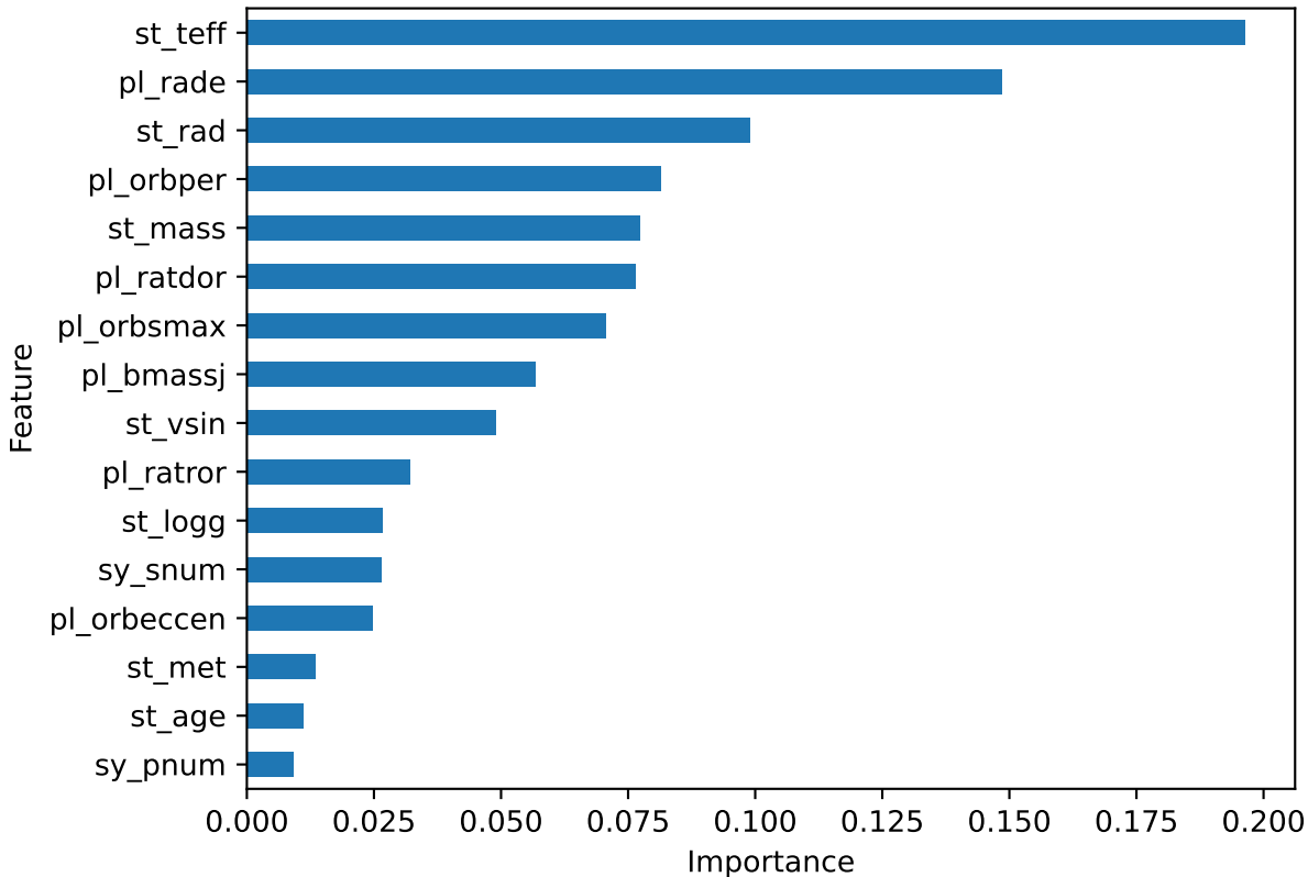
Feature Importances
