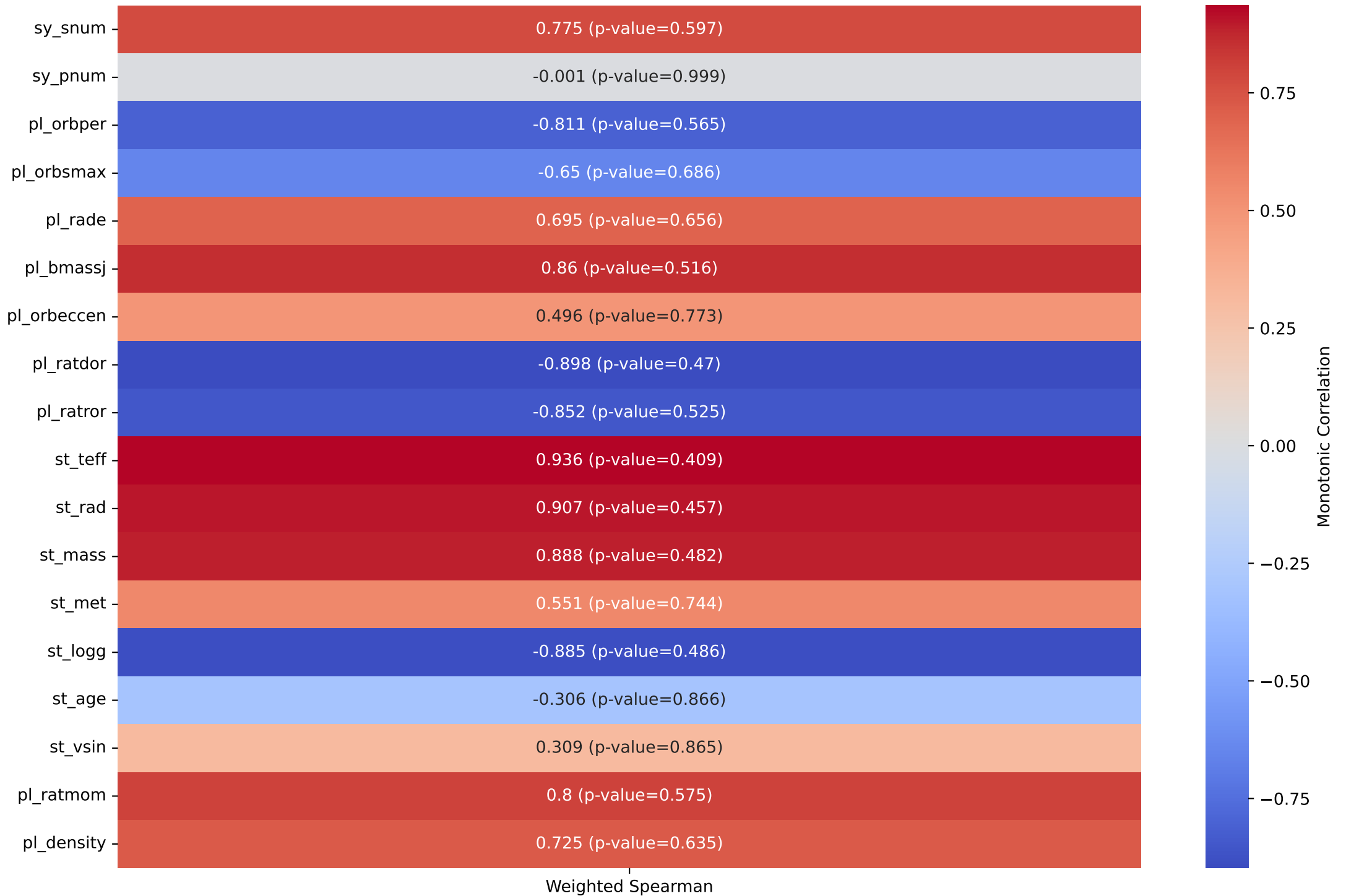
Weighted Spearman Monotonic Correlation Heatmap with p-values
