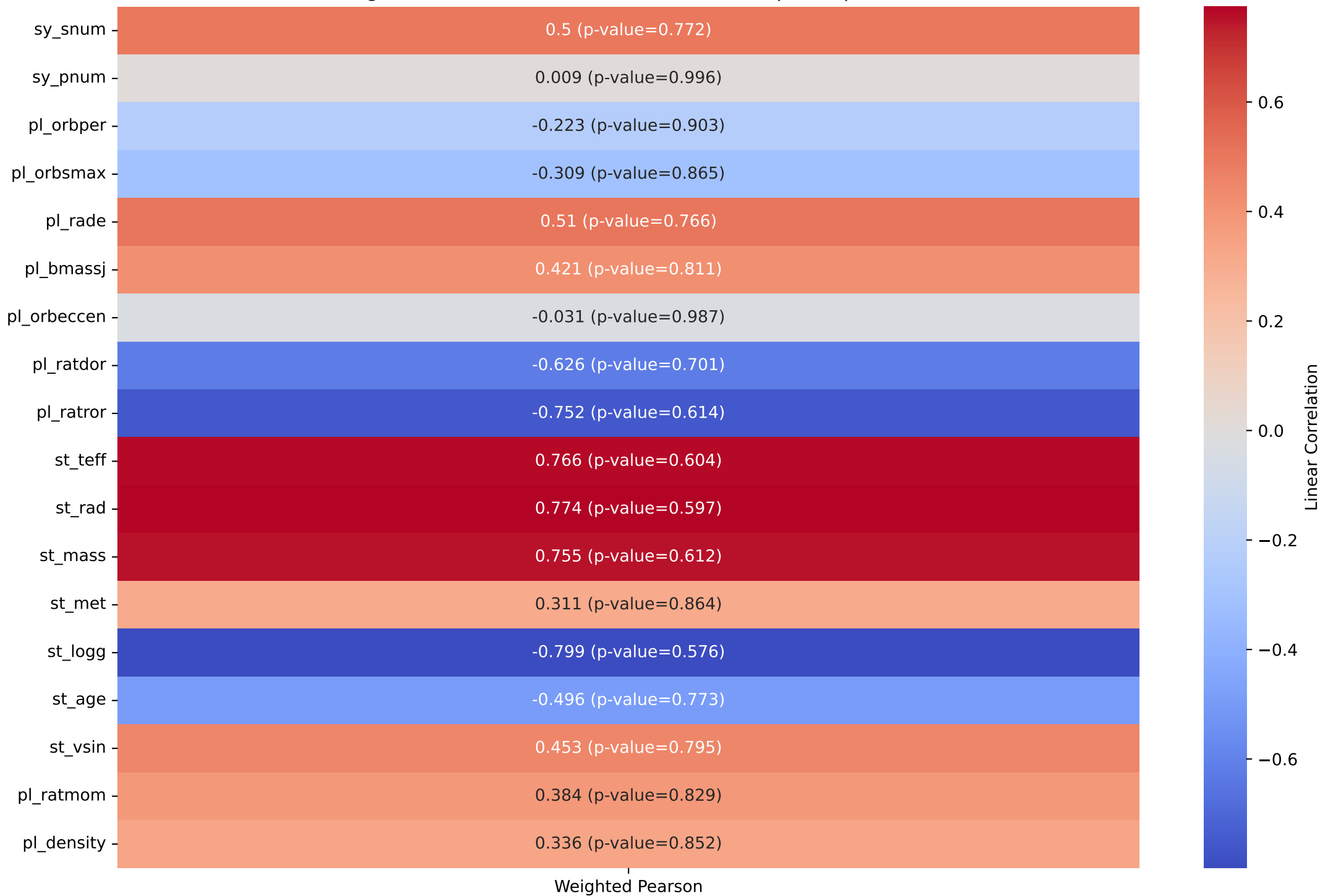
Weighted Pearson Linear Correlation Heatmap with p-values
